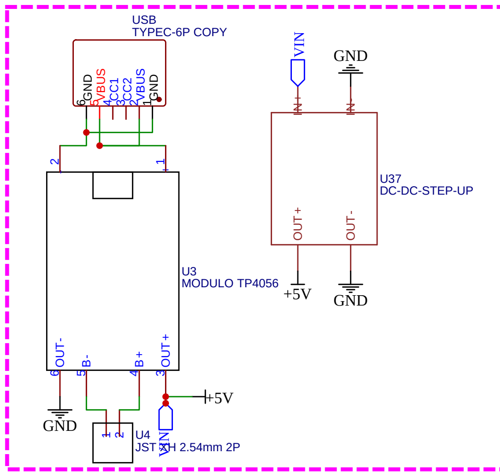
3.7v to 5v booster
